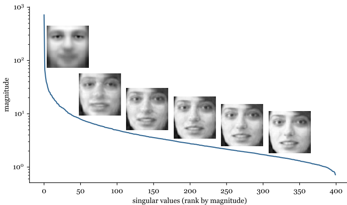
A plot of the singular values of the Olivetti faces data, in order of magnitude. The insets show the reconstructions using 10, 75, 140, 205, 270 and 335 singular values and vectors.
