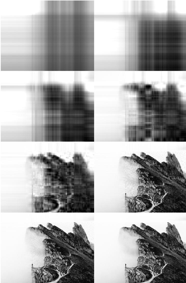
Reconstructions of our image using 1, 2, 3, 5, 10, 50, 100 and 500 singular values and vectors.
