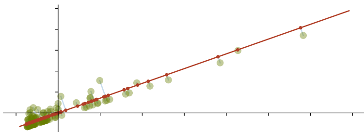
From Chapter 1: the first PC for a simple dataset.
